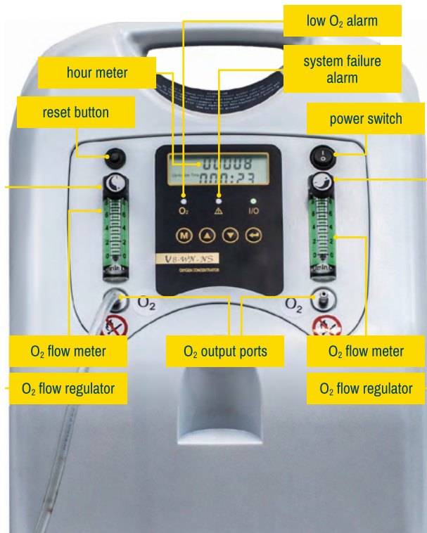
Fig 2.4.4a Front view of an oxygen Concentrator
