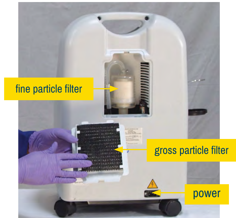
Fig 2.4.4b Back view of an oxygen Concentrator
